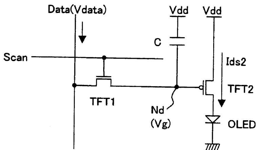
FIG. 2 CONVENTIONAL EXAMPLE
