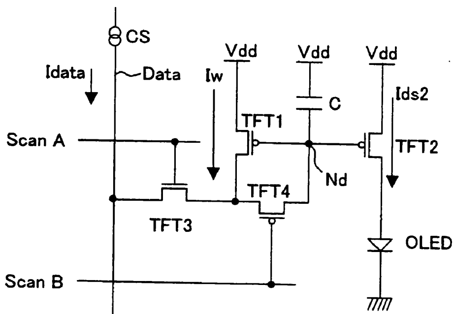
FIG. 3 CONVENTIONAL EXAMPLE
